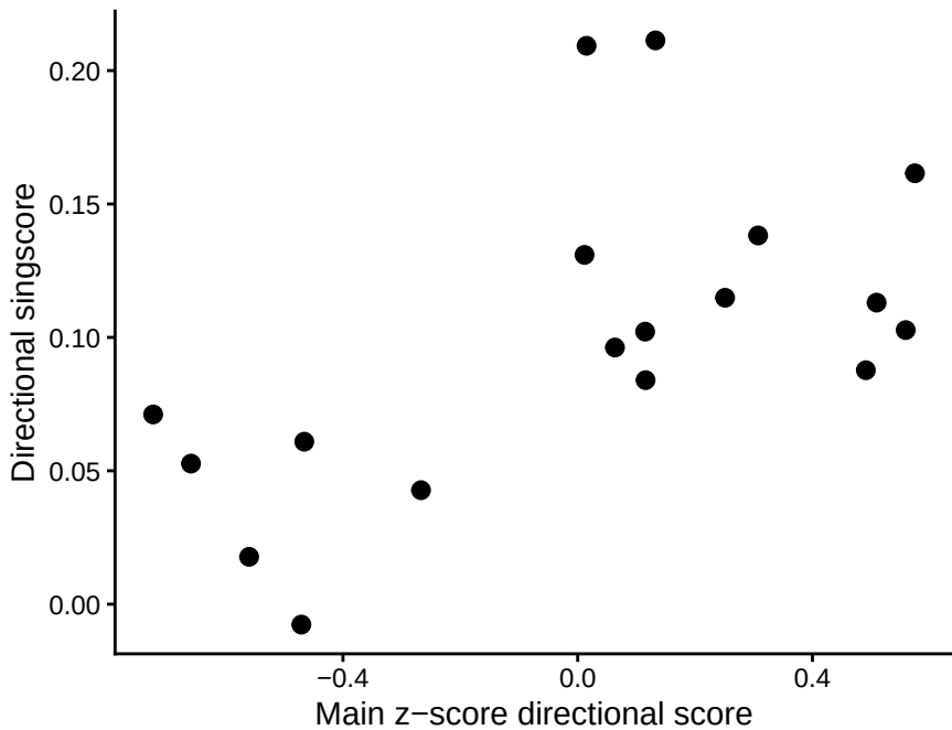
z-score score vs rank-based singscore
